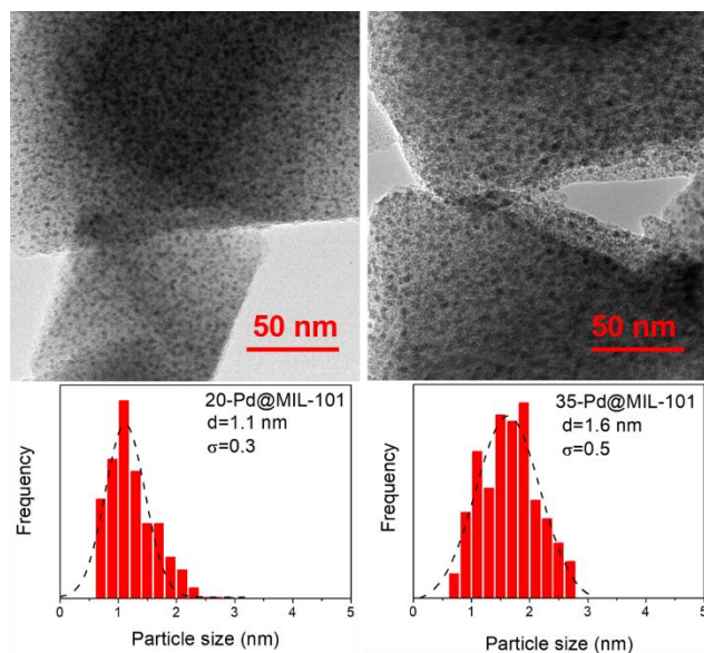
Figure 2. Selected TEM images with NPs size histograms of (left) 20-Pd@MIL-101 and (right) 35-Pd@MIL-101.
