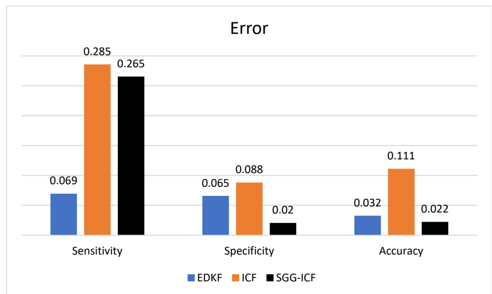
Figure 13. Error categorized by performance metric.
