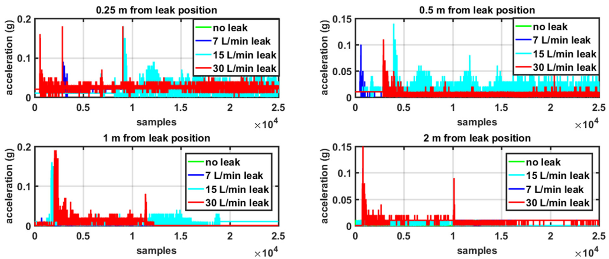
Figure 7. Leak characterization.
