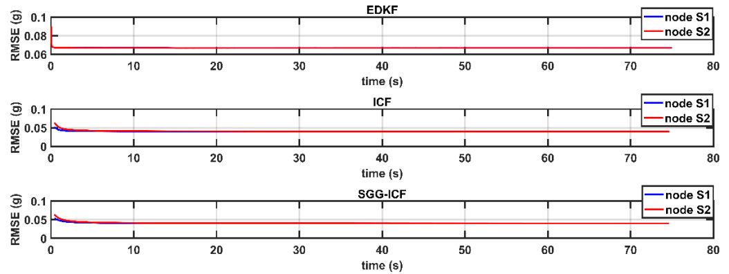
Figure 9. RMSE of the selected DKF algorithms.
