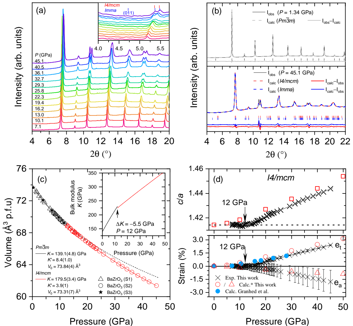
FIG. 2. (a) Diffraction patterns of sample S2. Inset: Zoom of the low-angle region. Low-angle fitted peak positions at 45.1 GPa are included as red and blue ticks corresponding to I4/mcm and Imma structures, respectively. Note that no diffraction peak is visible where the reflection (011) of an Imma phase would be expected. (b) Top: Rietveld fit (grey line) to a diffraction pattern (black line) acquired at 1.34 GPa. Bottom: Rietveld fit assuming tetragonal and orthorhombic phases (red and blue dashed lines, respectively) to a pattern acquired at a pressure of 45.1 GPa. Fitted positions for all reflections are included at the bottom as colored ticks. Both panels use the same intensity scale and residuals of the Imma fit are vertically shifted for a better comparison. (c) Pressure dependence of the volume per formula unit ABO 3 for the cubic and tetragonal phases (black and red, respectively). Lines are fits to BM EoS (for the cubic phase a high pressure extrapolation is included as a black dashed line). Inset: Bulk modulus as a function of pressure. (d) Top: Tetragonality ( c/a ratio) as a function of pressure as obtained from the fitted x-ray diffraction (XRD) patterns of sample S2 (crosses) and adapted DFT calculations (squares). Bottom: Volume ( e_a ) and tetragonal ( e_t ) spontaneous strains as obtained from the experiments (crosses), our calculations (open symbols) and calculations published by Granhed et al. [25]. Our reported DFT-values include a pressure shift (+10 GPa) as discussed in the text; this is not the case for values taken from Ref. [25] calculated through the hybrid Heyd-Scuseria-Ernzerhof (HSE) functional, which provides a slight larger volume than the one obtained from the WC-functional employed here (cf. Table I in Ref. [25]).
