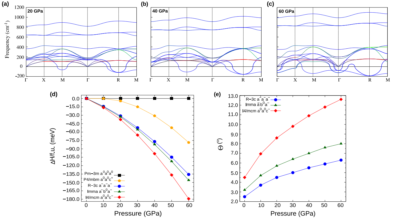
FIG. 3. (a,b,c) DFPT phonon dispersion curves in the cubic phase for 20, 40 and 60 GPa applied hydrostatic pressure (corresponding lattice parameters a are 4.049 Å, 3.955 Å and 3.883 Å, respectively). Red, green and blue phononic branches involve mostly Ba, Zr and O vibrations, respectively. (d) Computed enthalpies ( H ), with respect to the cubic phase taken as reference at each pressure. (e) Evolution of the oxygen octahedra rotation angle \Theta (in degree, °) with isotropic external pressure for different rotation patterns.
