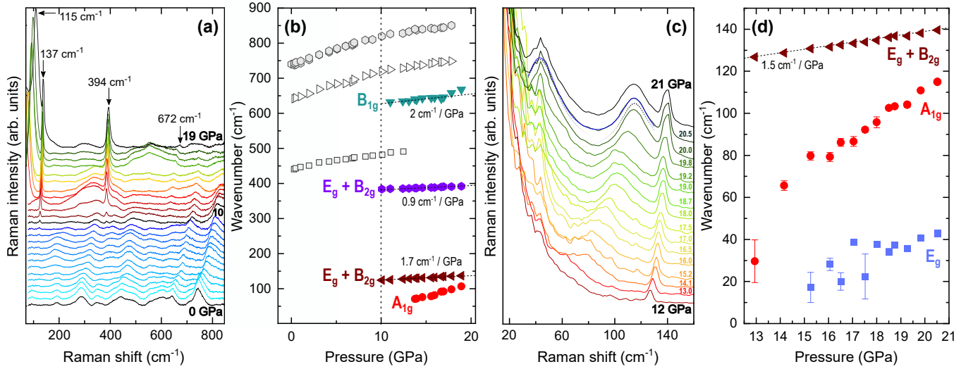
FIG. 1. Raman spectra of BaZrO 3 single crystals under pressure (a) from 0 to 19 GPa, when increasing the pressure, and (c) between 21 and 12 GPa, when releasing the pressure. The spectra in (a) are classical Stokes spectra, while the spectra in (c) are collected without cutting off the Rayleigh scattering of the laser line, allowing for observation of lower energies. An example of the Lorentzian fits performed on the Raman modes is shown in blue. (b) Pressure dependence of the wavenumbers of the phonon modes derived from the spectra obtained from 0 to 19 GPa, the solid symbols show the modes appearing above the transition at 10 GPa. (d) Behaviour of the two soft modes (and first hard mode) appearing above 10 GPa, these frequencies are derived from the spectra shown in (c), fitted with Lorentzian functions.
