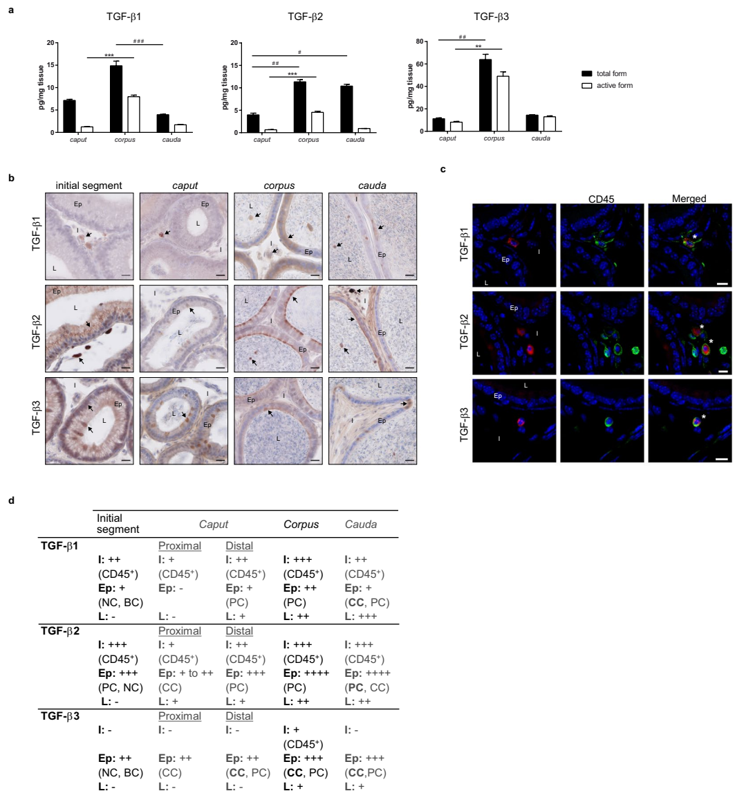
Figure 1. Quantification and localisation of the TGF-β isoforms in adult mice. (a) Concentrations of the total and active forms of the three TGF-β isoforms were determined by ELISA in the caput , corpus , and cauda epididymides of 5 month-old mice (pg/mg tissue). Bars represent means ± SEM. n = 7 (TGF-β1 and β2), n = 5 (TGF-β3). Kruskal-Wallis test. #Comparison between total forms: *P < 0.05, **P < 0.01, ***P < 0.001. *Comparison between active forms: **P < 0.01, ***P < 0.001. (b) Localisation of the TGF-β isoforms in the initial segment, caput , corpus , and cauda epididymides of adult mice. Arrows point to representative stained cells. L: lumen, Ep: epithelium, I: interstitium. Scale bars represent 20 μm. n = 10. (c) TGF-β-producing cells were identified based on their expression of the surface marker CD45 (pan-leucocyte, green). This immunostaining was done in combination with each isoform of TGF-β (A555, red). Only the corpus epididymis is shown and is representative of all segments of adult mice. *Show co-stained cells. L: lumen, Ep: epithelium, I: interstitium. Scale bars represent 10 μm. (d) Summary of the immunohistochemistry results presented in (b,c) . I: interstitium, Ep: epithelium, L: lumen, BC: basal cells, CC: clear cells, NC: narrow cells, PC: principal cells. -: absence of positive cells, +: low number of positive cells, ++: moderate number of positive cells, +++: high number of positive cells, ++++: very high number of positive cells. Cell density was visually determined.
