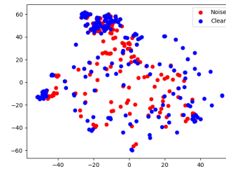
(b) ResNet
