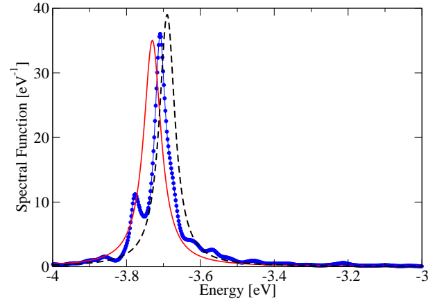
FIG. 1. Spectral function of a valence band state. This well represents the general trend of the majority of spectral functions covering the energy range involved in the absorption process, as discussed in the text. Blue line with dots is the calculated SF. This is compared with two Lorentzian functions corresponding to the OMS (red solid line) and to the QPA (black dash line). Both approximation reproduce the calculated SF quite well and the use of the OMS is, therefore, well motivated.
