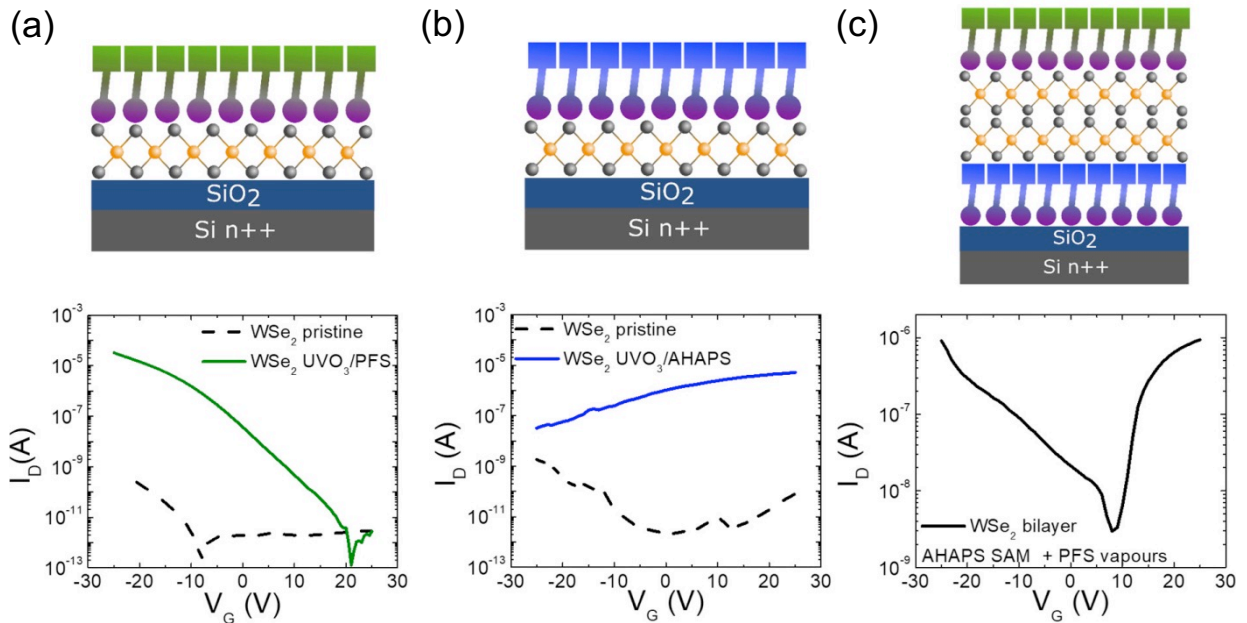
Figure 21. Device architecture and corresponding transfer curves of ozone treated \text{WSe}_2 single layer with (a) PFS vapor and (b) AHAPS vapor. For the sake of comparison, the transfer curves of the pristine \text{WSe}_2 single layers are also shown (dashed black lines). (c) Device architecture and corresponding transfer curve of bilayer \text{WSe}_2 after asymmetric functionalization: the bottom \text{WSe}_2 layer is in contact with AHAPS-treated \text{SiO}_2 dielectric, while the top \text{WSe}_2 layer was exposed to ozone and PFS vapor. Reproduced with permission from ref (333). Copyright 2019 American Chemical Society.
