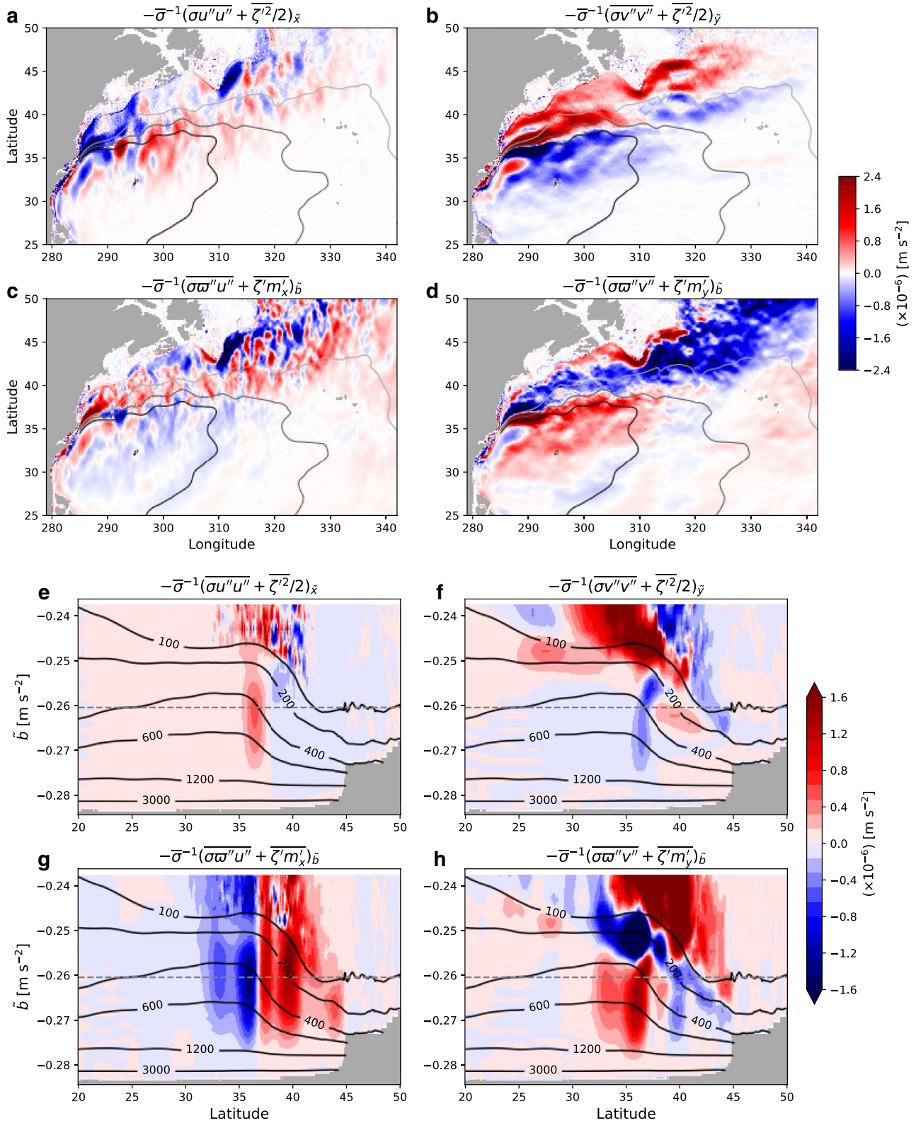
Figure 11. The annual mean of the convergence of eddy momentum flux and potential energy, and interfacial form stress for \bar{b} = -0.26 \text{ m s}^{-2} (a–d) The contours in gray shading east of 285°E indicate the 400, 300, and 200 m depth of the buoyancy surface. The annual and zonal mean transect between 290°E and 305°E of the E-P flux convergence is shown in colored shading and ensemble-mean depth in black contours (e–h). The iso-surface of buoyancy used through panels (a–d) is shown as the gray dashed line.
