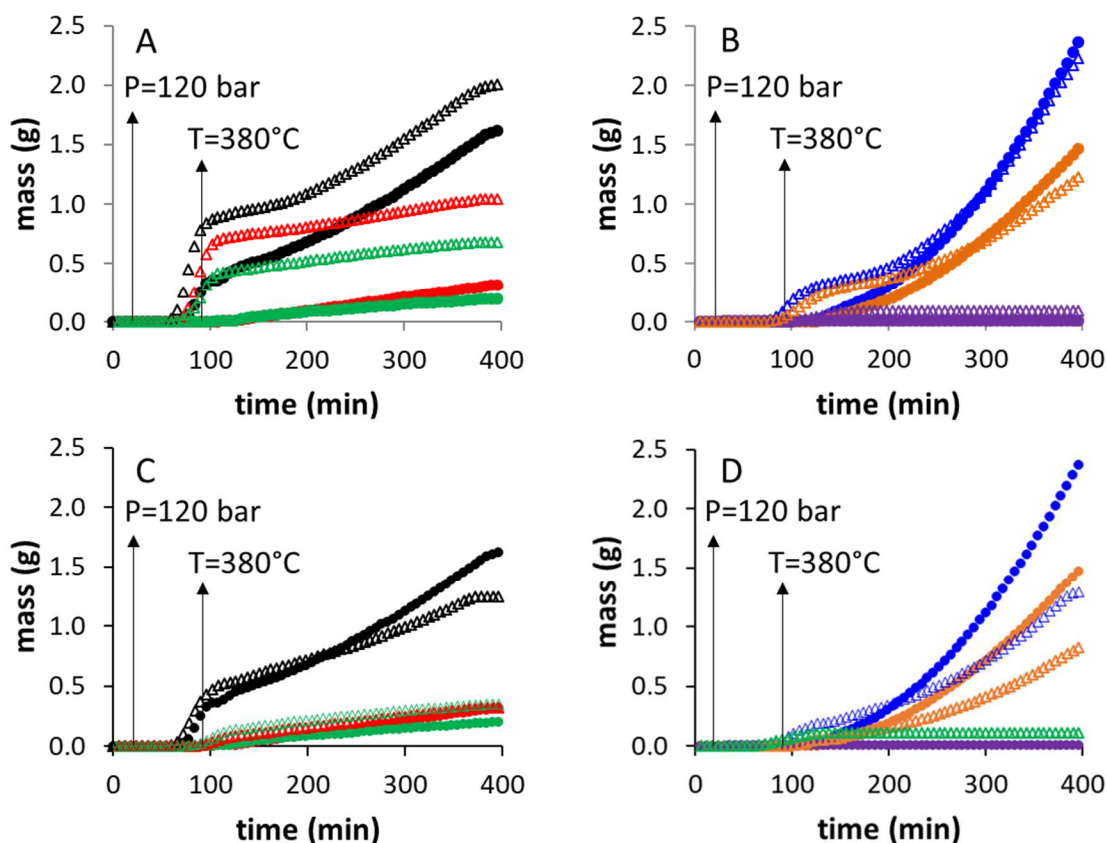
Fig. 4. Cumulative plots for gas phase analysis of light hydrocarbons for hydrocracking at 380°C and 120 bars H_2 . A: C1 VGO (●), C1 VGO/10% SPO (△), C2 VGO (●), C2 VGO/10% SPO (△), C3 VGO (●), C3 VGO/10% SPO (△). B: C4 VGO (●), C4 VGO/10% SPO (△), C5 VGO (●), C5 VGO/10% SPO (△), C6 VGO (●), C6 VGO/10% SPO (△). C: C1 VGO (●), C1 VGO/10% HTL (△), C2 VGO (●), C2 VGO/10% HTL (△), C3 VGO (●), C3 VGO/10% HTL (△). D: C4 VGO (●), C4 VGO/10% HTL (△), C5 VGO (●), C5 VGO/10% HTL (△), C6 VGO (●), C6 VGO/10% HTL (△).
