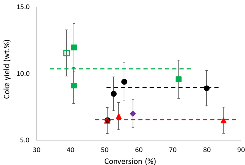
Fig. 9. Coke yield expressed as wt.% of catalyst mass for hydrocracking experiments of VGO and VGO + bio-liquid. Symbols: Experimental data; Green dashed line (top): trend for VGO/HTL, Black dashed line (middle): trend for VGO, Red dashed line (bottom): trend for VGO/SPO, SDPO. ●: VGO, ◆: VGO + 10 % SDPO, ■: VGO + 10% HTL, □: VGO + 20% HTL, ▲: VGO + 10% SPO, △: VGO + 20% SPO.
