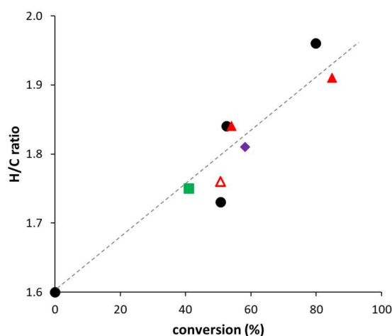
Fig. 3. H/C ratio versus 360 °C+ conversion. ●: VGO, ◆: VGO + 10% SDPO, ■: VGO + 10% HTL, ▲: VGO + 10% SPO, △: VGO + 20% SPO.
