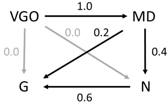
Fig. 10. 4-lump model for hydrocracking with VGO as feed, middle distillates (MD), naphtha (N) and gas (G) as products. The numbers close to the arrows are the values of the normalized rate constants.
