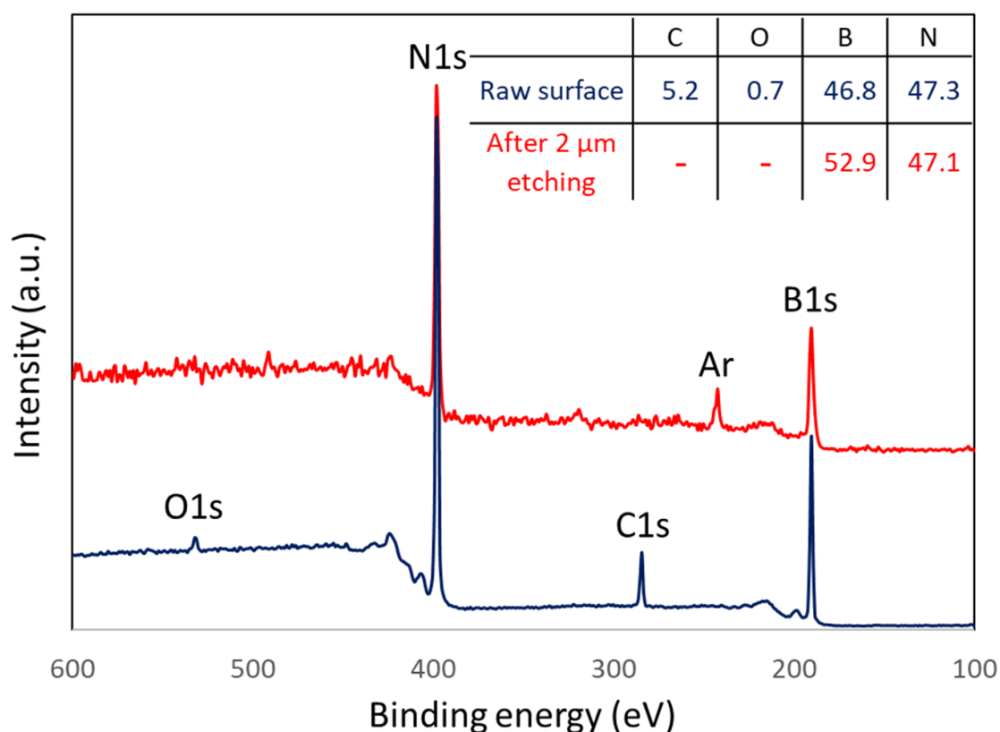
Figure 5. XPS general survey and elemental composition (inset) of hBN flake before (blue) and after (red) a 2 \mu\text{m} \text{Ar}^+ surface etching.
