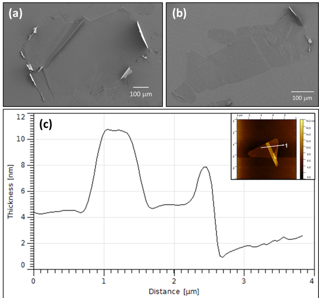
Figure 7. (a) and (b) SEM images of BNNSs of a few hundreds of microns as lateral size; (c) AFM profile obtained on BNNSs (inset).
