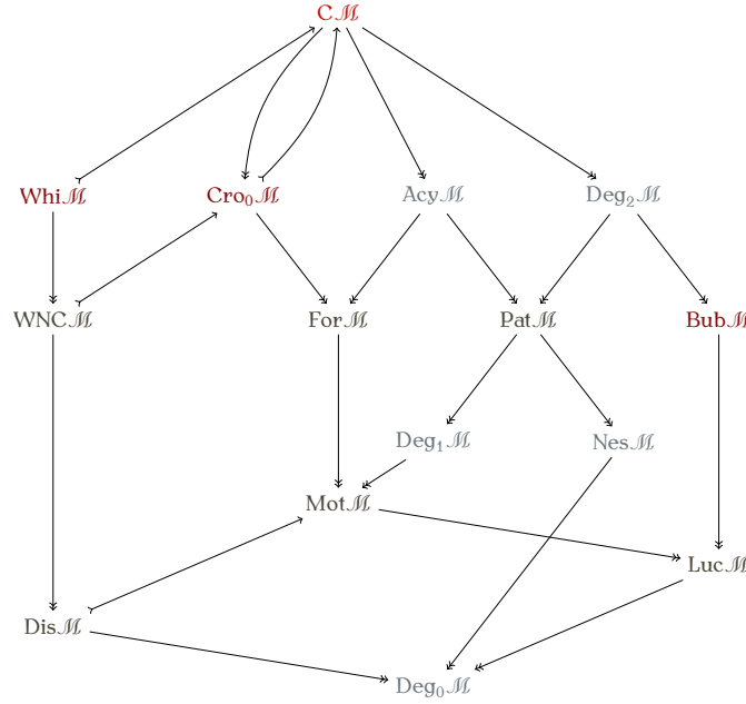
FIGURE 3. The diagram of the secondary suboperads and quotients of \text{C}\mathcal{M} together with some of their related main suboperads and quotients of \text{C}\mathcal{M} . Arrows \mapsto (resp. \twoheadrightarrow ) are injective (resp. surjective) operad morphisms. Here, \mathcal{M} is a unitary magma without nontrivial unit divisors.
