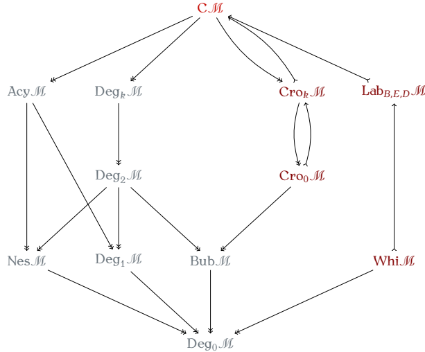
FIGURE 2. The diagram of the main suboperads and quotients of C\mathcal{M} . Arrows \dashrightarrow (resp. \rightarrow ) are injective (resp. surjective) operad morphisms. Here, \mathcal{M} is a unitary magma without nontrivial unit divisors, k is a positive integer, and B, E , and D are subsets of \mathcal{M} such that 1_{\mathcal{M}} \in B , 1_{\mathcal{M}} \in E , and E \star B \subseteq D .
