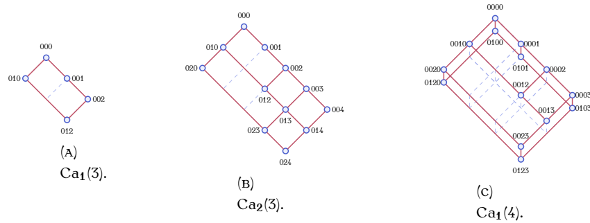
FIGURE 8. Hasse diagrams of some \delta -canyon posets.
