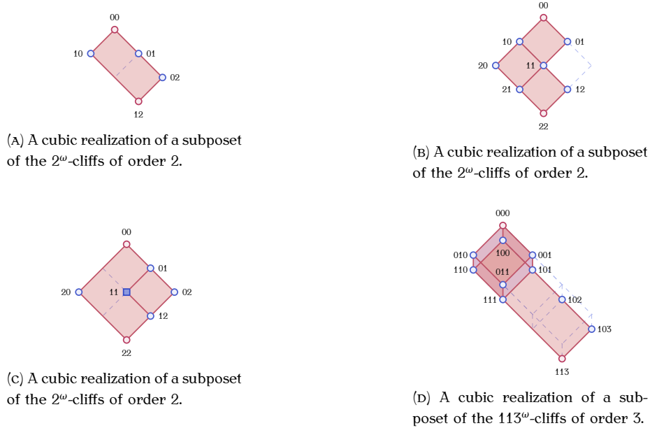
FIGURE 3. Some cubic realizations of straight subposets of posets of \delta -cliffs for certain range maps \delta .
