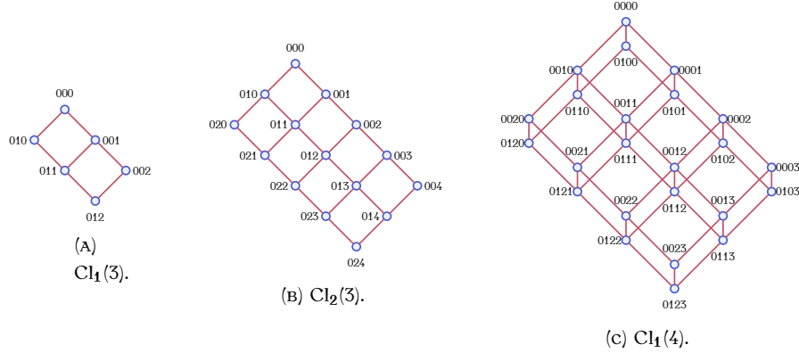
FIGURE 1. Hasse diagrams of some \delta -cliff posets.
