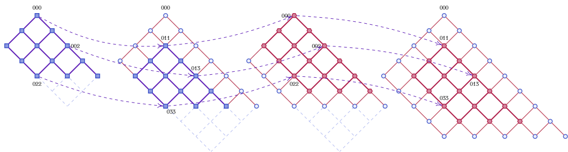
FIGURE 5. From the top to bottom and left to right, here are the posets Av_2(3) , Av_3(3) , Av_3(3) , and Av_4(3) . All these posets contain Av_2(3) as subset by restricting on input-wings, output-wings, or butterflies.
