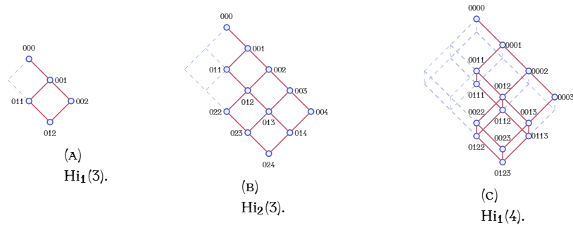
FIGURE 6. Hasse diagrams of some \delta -hill posets.
