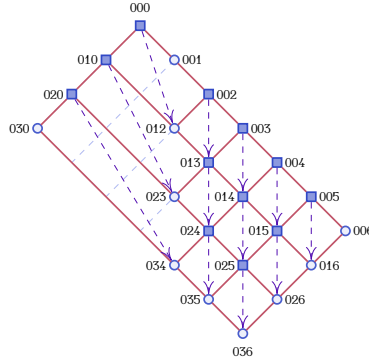
FIGURE 10. The poset \text{Ca}_3(3) wherein output-wings are marked. The arrows connect these elements to their images by the bijection \rho .
