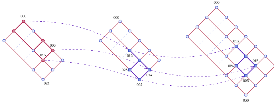
FIGURE 11. From the top to bottom and left to right, here are the posets \text{Ca}_2(3) , \text{Ca}_2(3) , and \text{Ca}_3(3) . The two last posets contain \mathcal{G}(\text{Hi}_1)(3) as subposets. There is a poset morphism between the output-wings of the first one and the input-wings of the second one.
