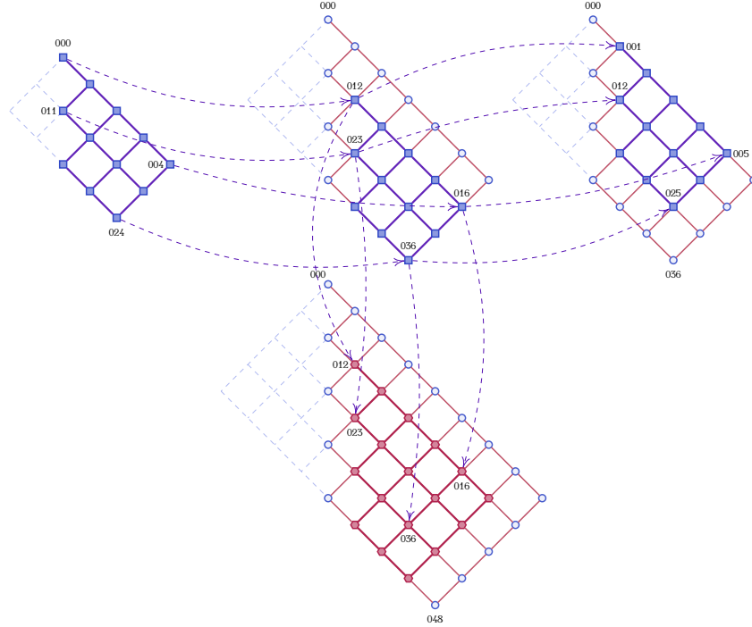
FIGURE 7. From the top to bottom and left to right, here are the posets \text{Hi}_2(3) , \text{Hi}_3(3) , \text{Hi}_3(3) , and \text{Hi}_4(3) . All these posets contain \text{Hi}_2(3) as subposet by restricting on input-wings, output-wings, or butterflies.
