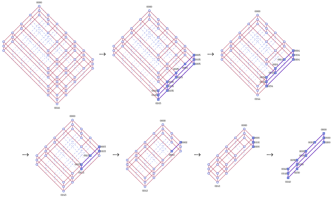
FIGURE 9. A sequence of interval contractions from \text{Ca}_2(4) to a poset isomorphic to \text{Ca}_2(3) . These interval contractions are poset derivations as introduced in Section 1.3.4. The marked intervals are the ones involved in the interval doubling operations.
