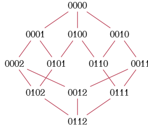
FIGURE 2. The Hasse diagram of the poset (\text{Cl}_{0112^\omega}(4), \preceq') .
