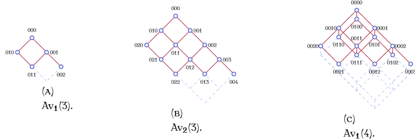
FIGURE 4. Hasse diagrams of some \delta -avalanche posets.
