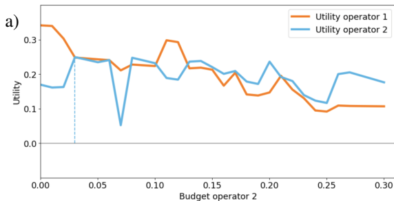
Fig. 3. a) Evolution of M(s_1, s_2) with s_1 = 0.0 and s_2 \in [0.0, 0.3] . b) Utility of the first player M_1(s_1, s_2) for s_1 = 0.0 and s_2 \in [0.0, 0.3] , and its upper bound u_1^{VS}(s_1, s_2) with s_1 = \{0.1, 0.2, 0.3, 0.4, 0.5\} and s_2 \geq 0.0 . The strategies s_1 \in \{0.3, 0.4, 0.5\} are dominated by the strategy s_1 = 0.0 .
