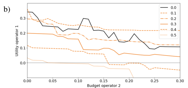
Fig. 3. a) Evolution of M(s_1, s_2) with s_1 = 0.0 and s_2 \in [0.0, 0.3] . b) Utility of the first player M_1(s_1, s_2) for s_1 = 0.0 and s_2 \in [0.0, 0.3] , and its upper bound u_1^{VS}(s_1, s_2) with s_1 = \{0.1, 0.2, 0.3, 0.4, 0.5\} and s_2 \geq 0.0 . The strategies s_1 \in \{0.3, 0.4, 0.5\} are dominated by the strategy s_1 = 0.0 .
