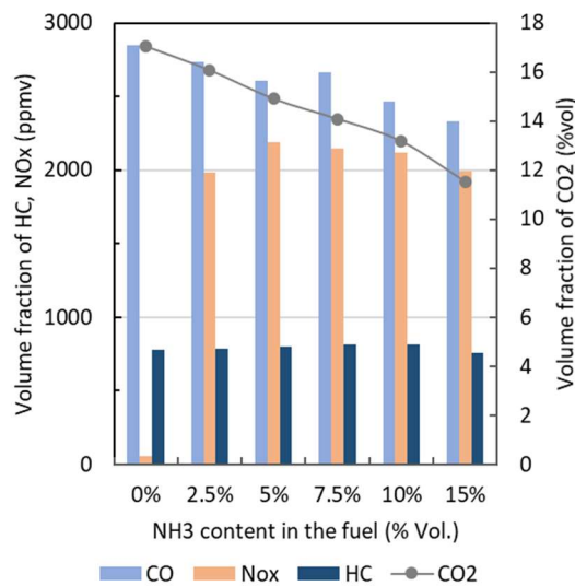
Figure 13: Evolution of syngas emissions as function of ammonia content at 1 bar intake pressure
