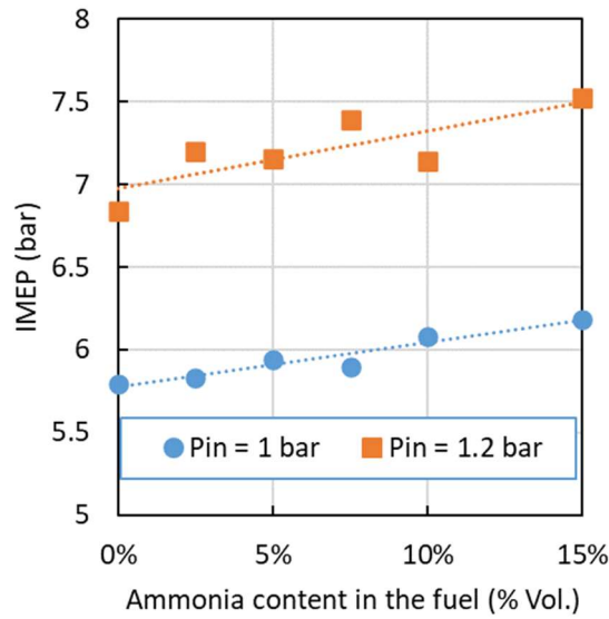
Figure 8: IMEP of syngas as a function of the ammonia content for both intake pressures – \phi=1
