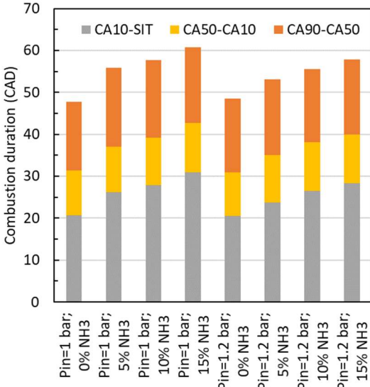
Figure 11: Combustion duration analysis of syngas as a function of the ammonia content in the blend for both intake pressures – \phi=1
