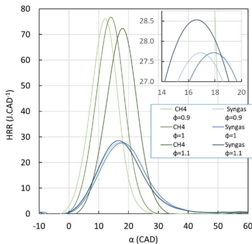
Figure 4: Net heat release rate of syngas and methane for several equivalence ratios at 1 bar intake pressure
