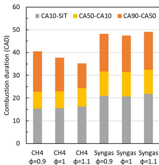
Figure 5: Combustion duration analysis comparing methane and syngas as a function of the equivalence ratio at 1 bar of intake pressure
