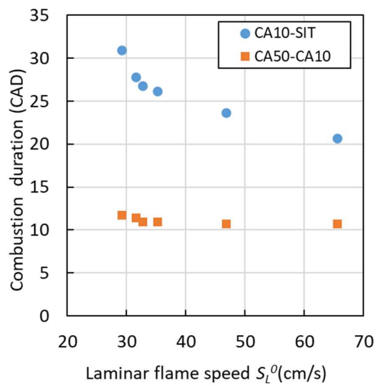
Figure 12: Combustion duration as function of the laminar flame speed calculated at SIT conditions and for intake pressure of 1 bar – \phi=1
