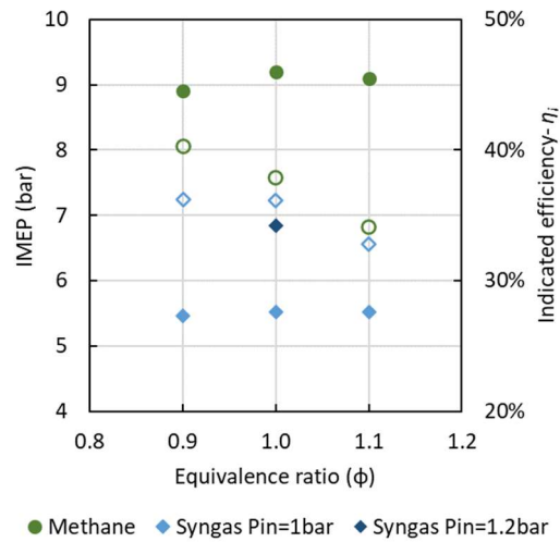
Figure 3: IMEP (filled symbols) and Indicated efficiency (empty symbols) of syngas compared to methane as a function of the equivalence ratio
