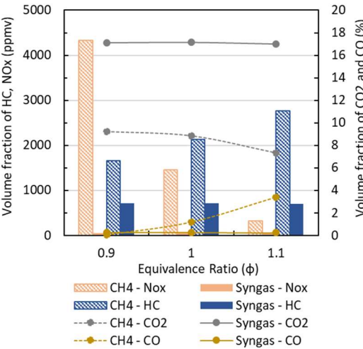
Figure 6: Comparison of exhaust emissions for syngas and pure methane for 3 equivalence ratios at 1 bar of intake pressure
