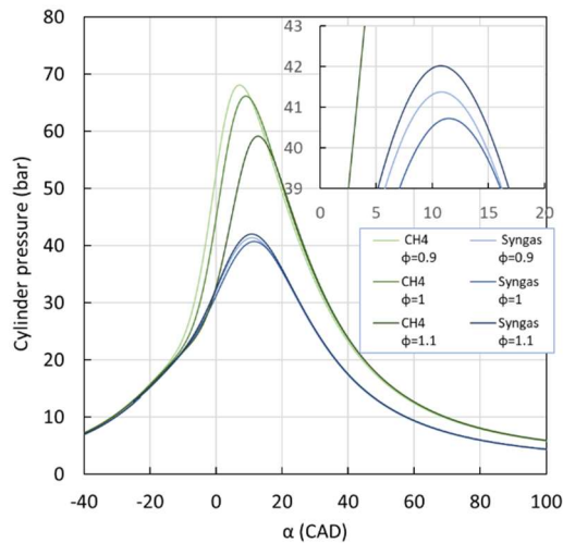
Figure 2: In-cylinder pressure evolution for syngas compared to pure methane for three equivalence ratios at 1 bar intake pressure.
