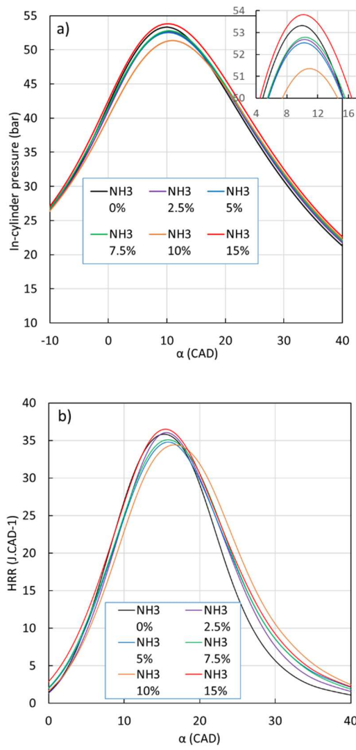
Figure 7: In-cylinder pressure (a) and HRR evolution as a function of ammonia content (%Vol). in the syngas/ammonia blend at 1.2 bar intake pressure – \phi=1
