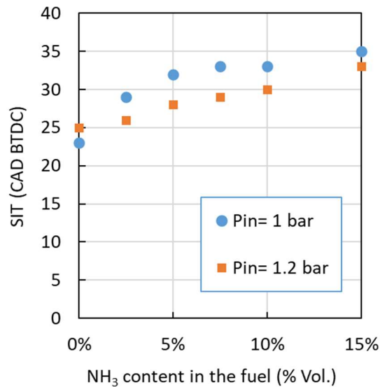
Figure 9: Optimised SIT as a function of ammonia content in syngas for two intake pressures – \phi=1
