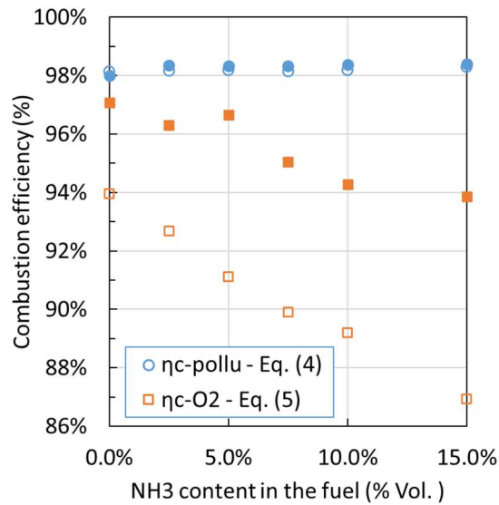
Figure 14: Combustion efficiency of syngas as a function of ammonia content calculated from Eq.4 and 5.
