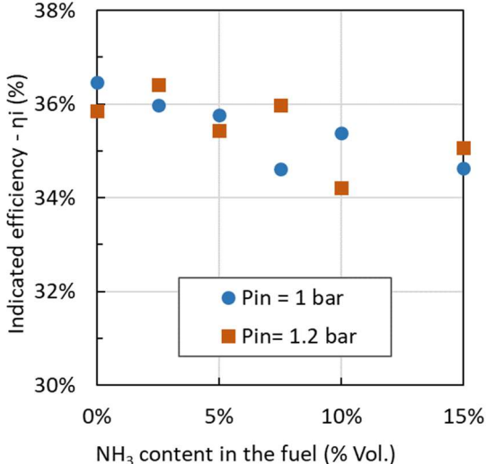
Figure 10: Indicated efficiency as a function of ammonia content in the blend for both intake pressures – \phi=1
