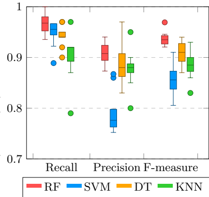
Fig. 2: Cross validation distribution
