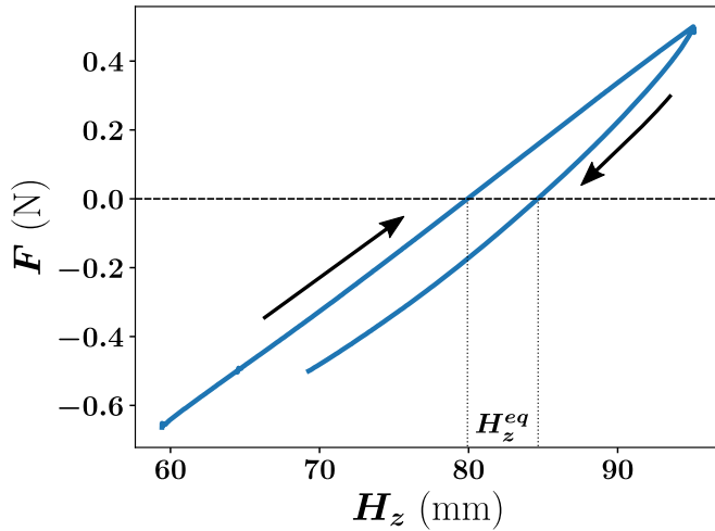
FIG. 9. Force-displacement response of the stack of four modules studied in Sec. III B near the rest position for the configuration 0000. The dotted lines represent the limit values of H_z^{eq} that we used in Fig. 7.
