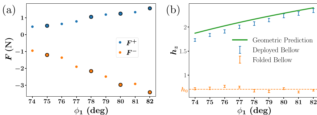
FIG. 4. (a) Force thresholds with respect to the pattern angle \phi_1 . The four highlighted modules are those used in Sec. III B. (b) Normalized height h_z = \frac{h}{\ell_1} measured for the folded and deployed configurations. The solid green line corresponds to the geometrical prediction of the deployed height given by (3). The dashed orange line corresponds to the mean value h_0 = 0.70 measured for the folded height.
