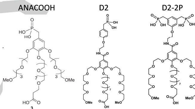
Figure 1 : Scheme of the earlier used dendron ANACOOH and of dendron molecules used to functionalize the NPs
