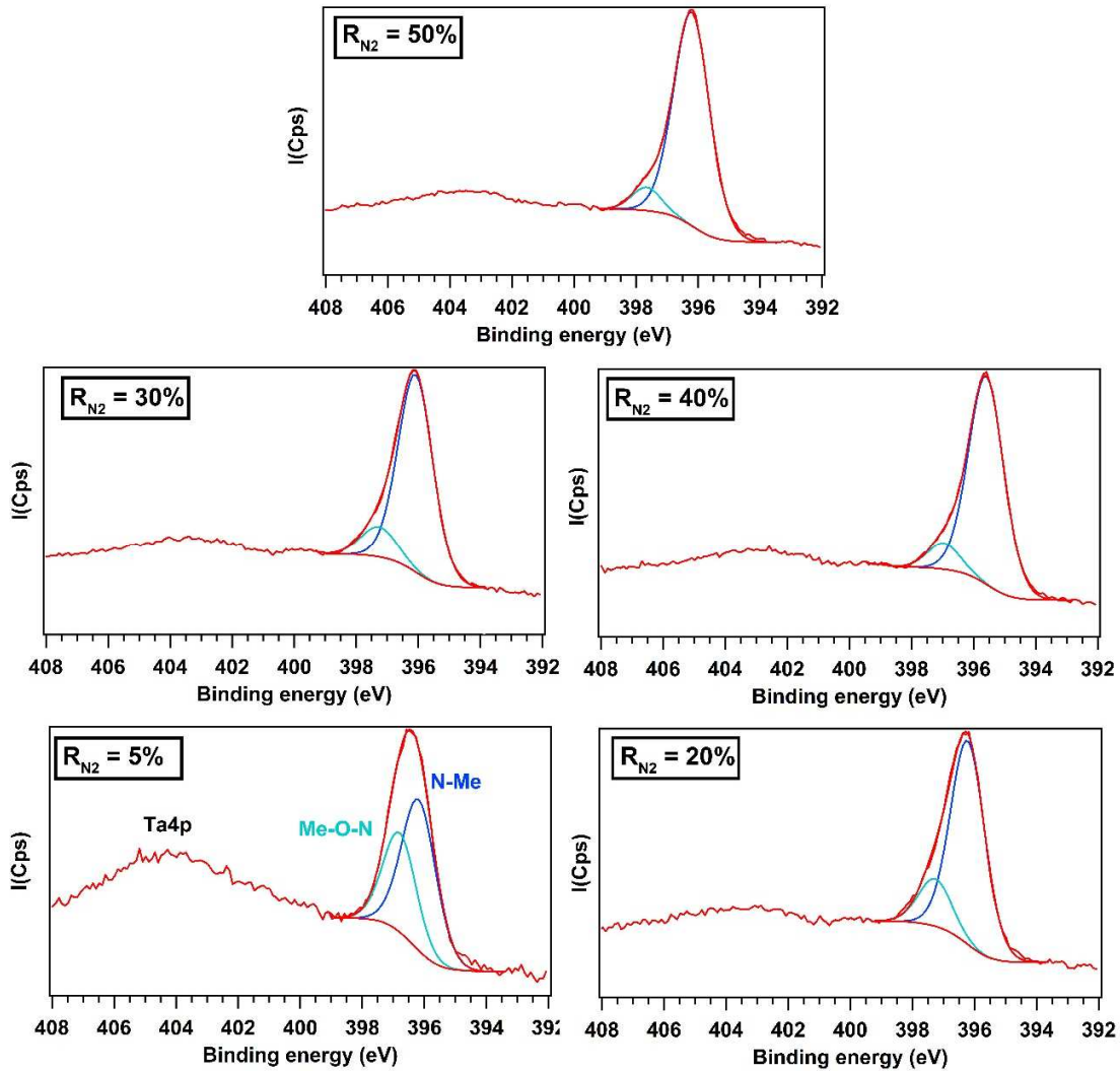
Figure 2. N1s XPS spectra of AlTiTaZrHf(-N) as a function of R_{N_2}
