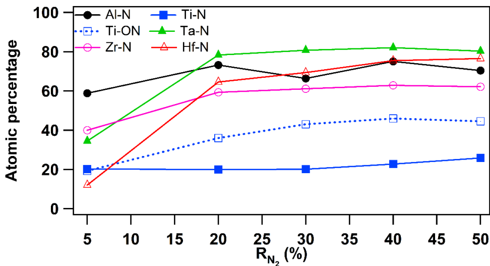
Figure 5. Atomic percentage of individual elements of AlTiTaZrHf(-N) films as a function of R_{N_2} according to XPS analysis.
