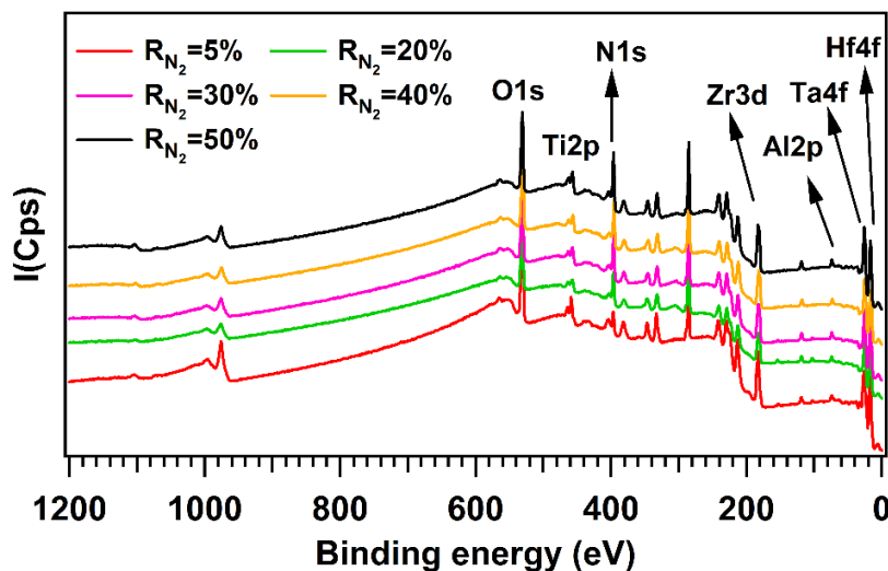
Figure 1. XPS survey spectra of AlTiTaZrHf(-N) as a function of R_{N_2}
