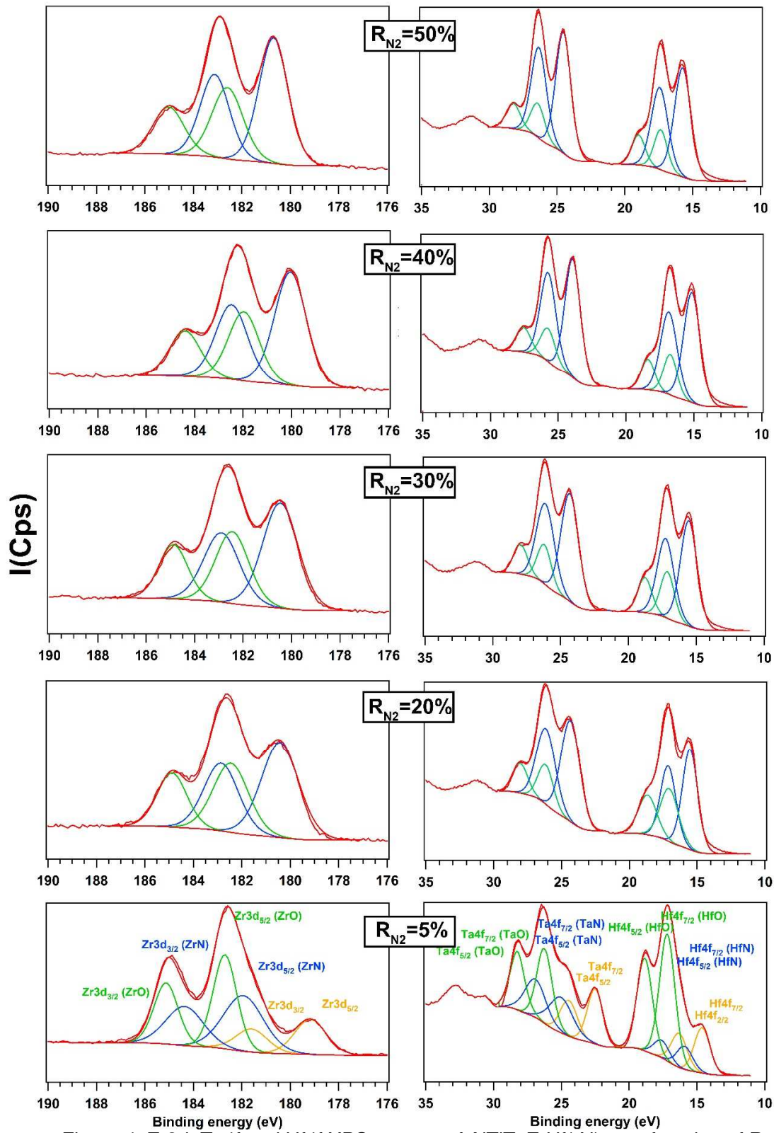
Figure 4. Zr3d, Ta4f and Hf4f XPS spectra of AlTiTaZrHf(-N) as a function of R_{N_2}
