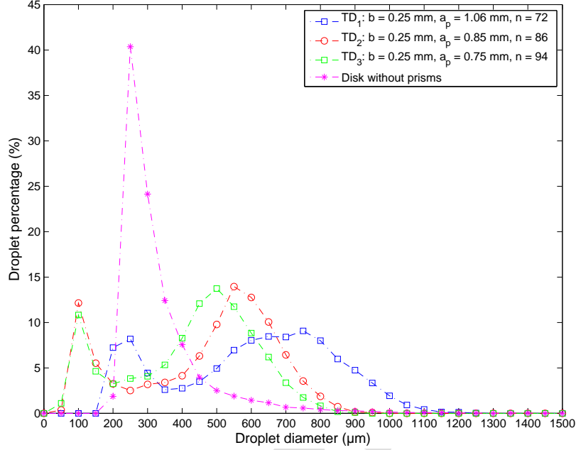
FIG. 18: Representation of droplet percentages as a function of their diameters in the case of three designs TD_1 , TD_2 and TD_3 . The prisms are placed at R_p = 15 mm from the jet impact. The curve disk without prisms corresponds to droplets emitted from the Savart sheet. All the measurements were performed for Q = 2.8 \cdot 10^{-5} \text{ m}^3 \cdot \text{s}^{-1} .
