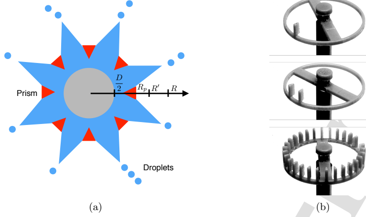
FIG. 4: (a) Top view of the non-laminar Savart sheet perturbed by triangular prisms. (b) Pictures from the side of the structures used to control the non-laminar sheet. Single triangular prism (top), two triangular prisms (middle) and N triangular prisms (bottom).
