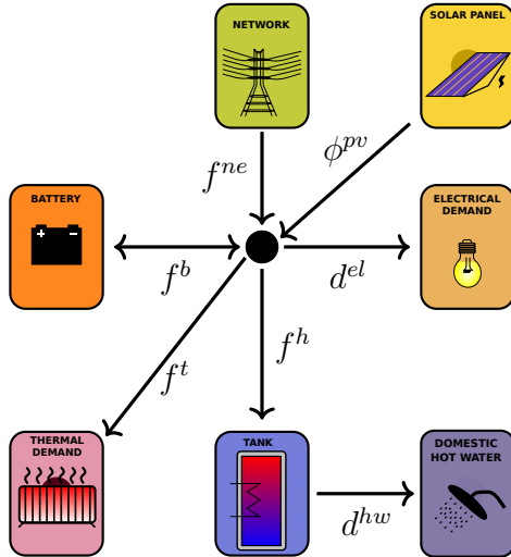
Figure 1: Electrical microgrid
