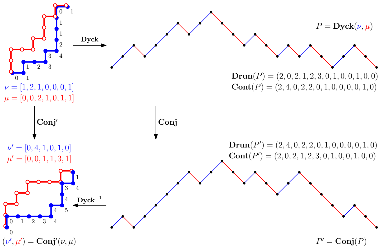
Figure 6: Example of the bijections Conj and Conj' and how they transform the statistics Cont and Drun . The reverse horizontal distances of points on the lower paths are also given.
