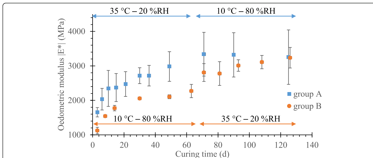
Fig. 5 Mean stiffness evolution of groups A and B with time, tested at 15 °C, 10 Hz and 9.5 kN. The error bars represent the standard deviation on the three samples for group A and two for group B .
