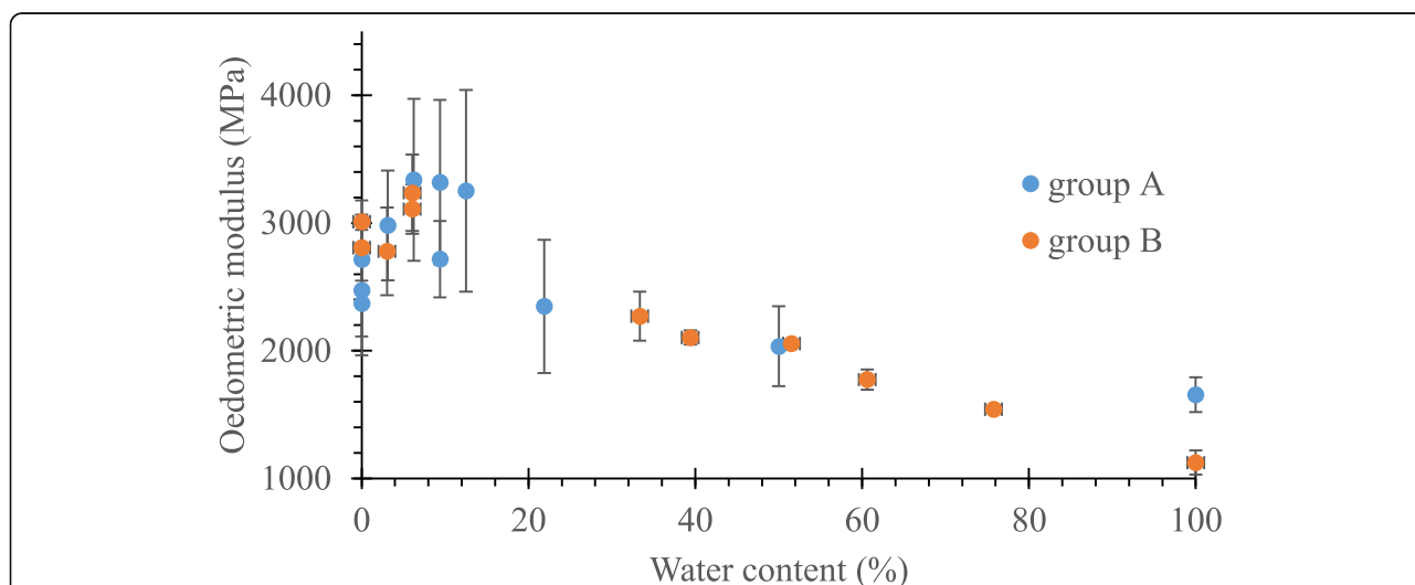
Fig. 6 Mean stiffness evolution of groups A and B versus mean water content, modulus tested at 15 °C, 10 Hz and 9.5 kN. The error bars represent the standard deviation on the three samples for group A and two for group B . Once again, we suppose that when the water content is minimal, the samples are dry.
