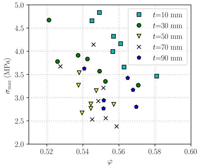
Figure 9: Failure stress as a function of pore volume fraction obtained experimentally.
