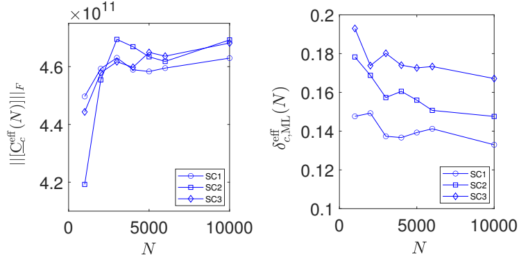
Figure 4: For scale separation, SC1, SC2, and SC3, graph of N \mapsto \|[\underline{C}_c^{\text{eff}}(N)]\|_F (left figure) and N \mapsto \delta_{c,ML}^{\text{eff}}(N) (right figure), computed with the constrained learned set.
