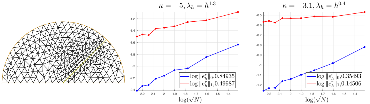
Figure 4: A given mesh (left). Behavior of the relative L^2 and H_0^1 errors with respect to the mesh-size h \sim \sqrt{N} , where N is the total number of nodes of the mesh, with the observed convergence rates in the caption, when \kappa_\varepsilon = -5 (center) and \kappa_\varepsilon = -3.1 (right).
