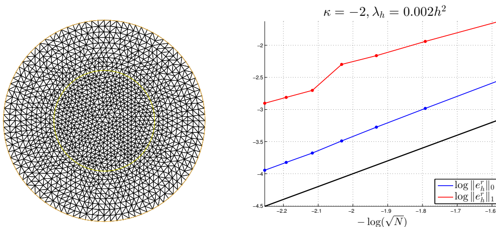
Figure 3: A given mesh (left). Behavior of the relative L^2 and H_0^1 errors with respect to the meshsize h \sim \sqrt{N} , where N is the total number of nodes of the mesh (right)
