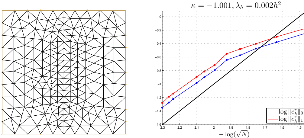
Figure 2: A given mesh (left). Behavior of the relative L^2 and H_0^1 errors with respect to the meshsize h \sim \sqrt{N} , where N is the total number of nodes of the mesh (right).
