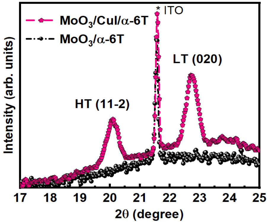
Fig. 5. XRD patterns of \alpha -6T films deposited on ITO/MoO 3 and ITO/MoO 3 /CuI(1.5 nm)
