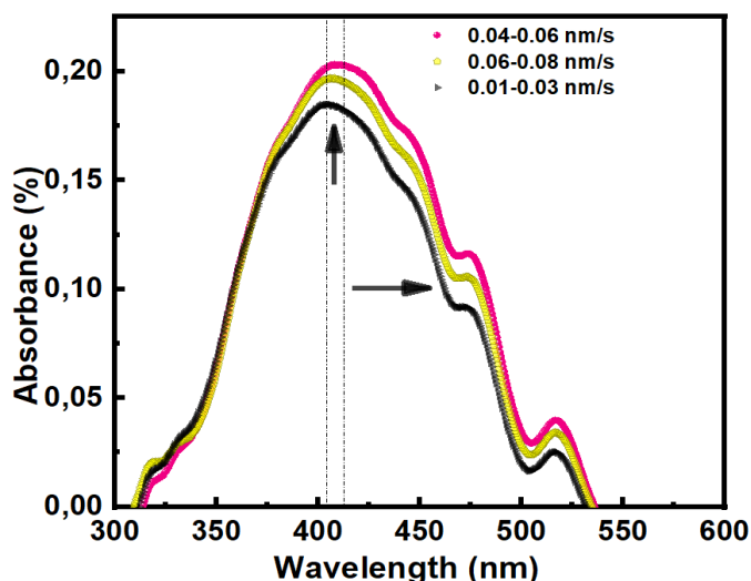
Fig. 4. Optical density spectra of \alpha -6T films deposited with low speed (0.01-0.03 nm/s), medium speed rate (0.04 – 0.06 nm/s) and fast speed rate (0.06-0.08 nm/s).
