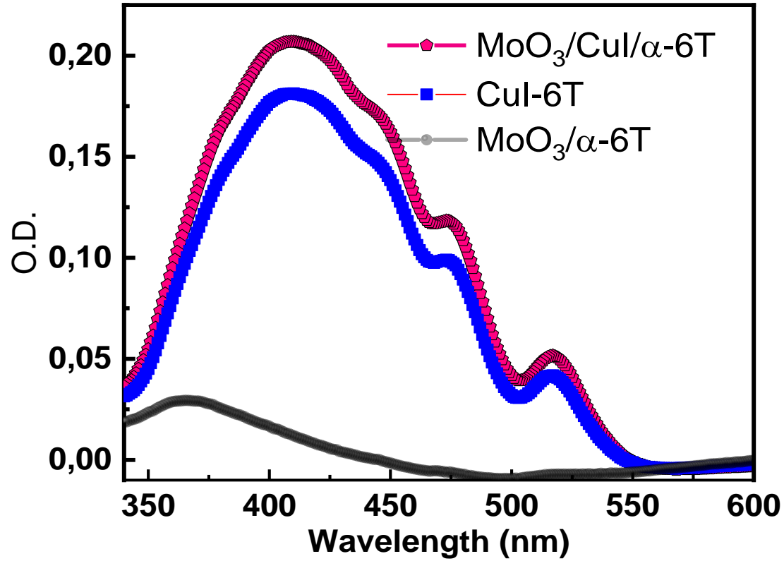
Fig. S2. Optical density spectrums of \alpha -6T films deposited on \text{MoO}_3 , \text{MoO}_3/\text{CuI}(1.5 \text{ nm}) and CuI HTLs
