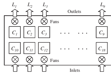
Fig. 2. The layout of the RECS server system.
