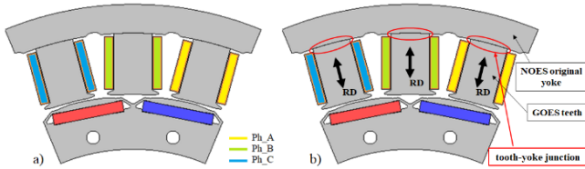
Fig. 15. Stator tooth segmentation: a) NOES reference motor, b) GOES teeth motor
