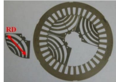
Fig. 13. SRM with GOES segmented rotor [26]
