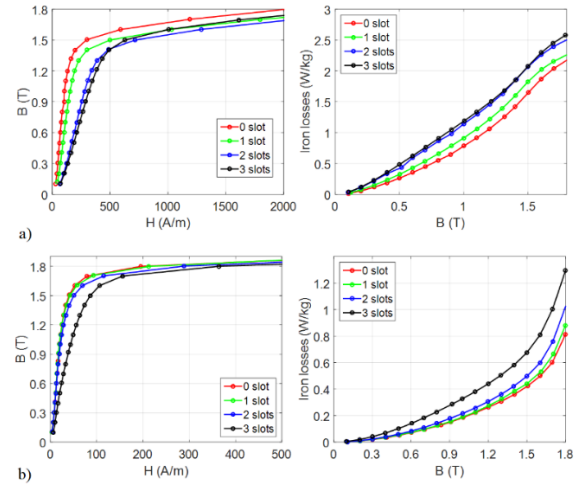
Fig. 7. Epstein measurements of magnetic performances, B-H curves and specific losses at 50Hz: a) NOES sheets, b) GOES sheets width)
