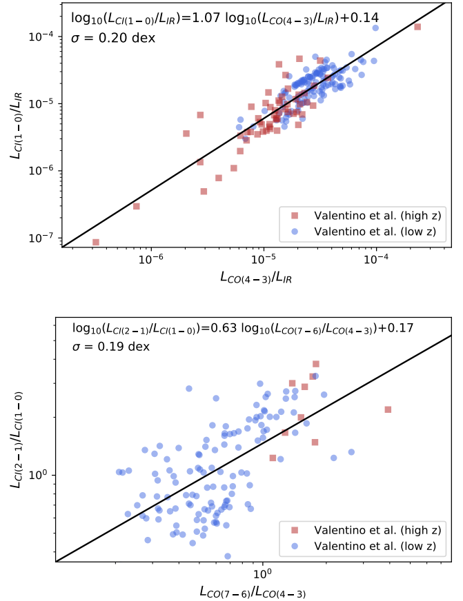
Fig. 1. Empirical relations used to produce the [CI] line fluxes. Upper panel: relation between the L_{\text{[CI](1-0)}/L_{\text{IR}} and L_{\text{CO}(4-3)}/L_{\text{IR}} ratios. The filled blue circles and the red filled squares are, respectively, the low- z and high- z galaxies compiled by Valentino et al. (2020b) . The solid line is our best-fit of this correlation used to generate [CI](1–0) fluxes in our simulation. Lower panel: same figure for the relation between the L_{\text{[CI](2-1)}/L_{\text{[CI](1-0)}} and L_{\text{CO}(7-6)}/L_{\text{CO}(4-3)} ratios.
