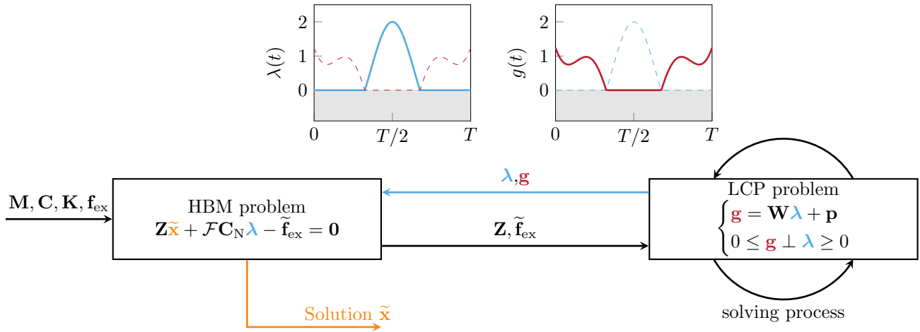
Figure 5. LCP-HBM procedure.
