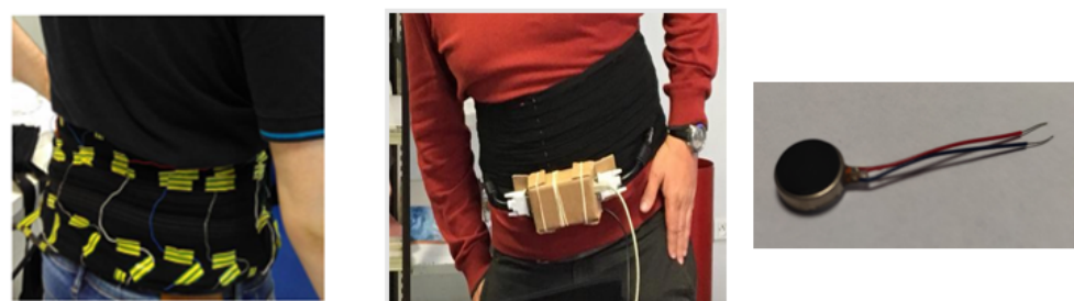
Figure 7. TactiBelt prototype ( left , showing vibrator positions, and center , showing the complete device) and type of used vibrator ( right , RS DC minivibration motor).
