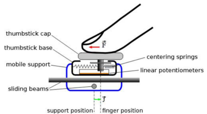
FIGURE 2. A flat thumbstick is placed on top of the mobile support (in blue) to acquire user's intended movement. As the user manipulates the thumbstick cap, the difference \vec{J} between the finger's position and the support's position is measured. The motion control moves then the mobile support to follow user's finger. By inducing offsets in this motion control, it is possible to set a predefined offset in the position difference \vec{J} . The centering springs of the thumbstick apply a force that is nearly proportional to the offset, allowing to control the force experienced by the user.
