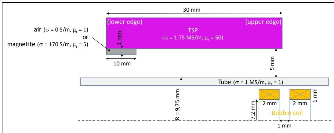
Figure 2. Simplified geometry for the simulation of bobbin coil signals for axisymmetric TSP with axisymmetric magnetite clogging-up.
