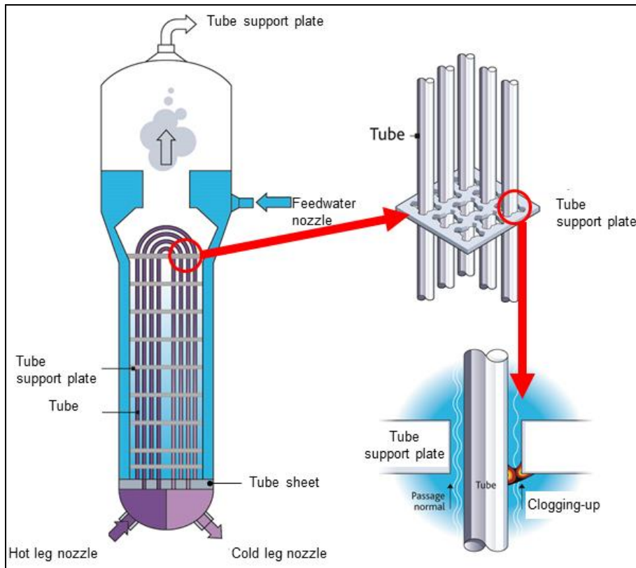
Figure 1. Tube support plate clogging-up. Corrosion products may build up in flow holes and modify the flow distribution (simplified deposit geometry).
