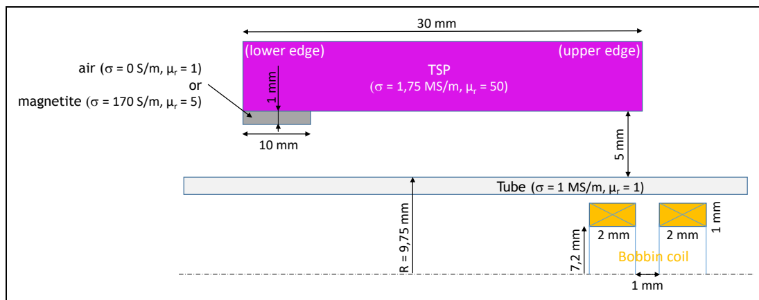
Figure 2. Simplified geometry for the simulation of bobbin coil signals for axisymmetric TSP with axisymmetric magnetite clogging-up.
