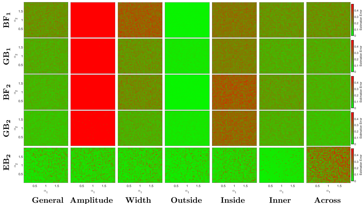
Figure 1: Map of (\alpha_1, \alpha_2) absolute estimation Error for each estimation method in row : Baseline Free (BF), Gaussian Baseline (GB), and Estimated Baseline (EB). Each column represent the same baseline dataset defined in Table 1. Each map has been computed by 100000 drawings equally split in 100x100 bins. The more red is the color, the greater the absolute error of estimation and the greener the color, the lower the absolute error of estimation.
