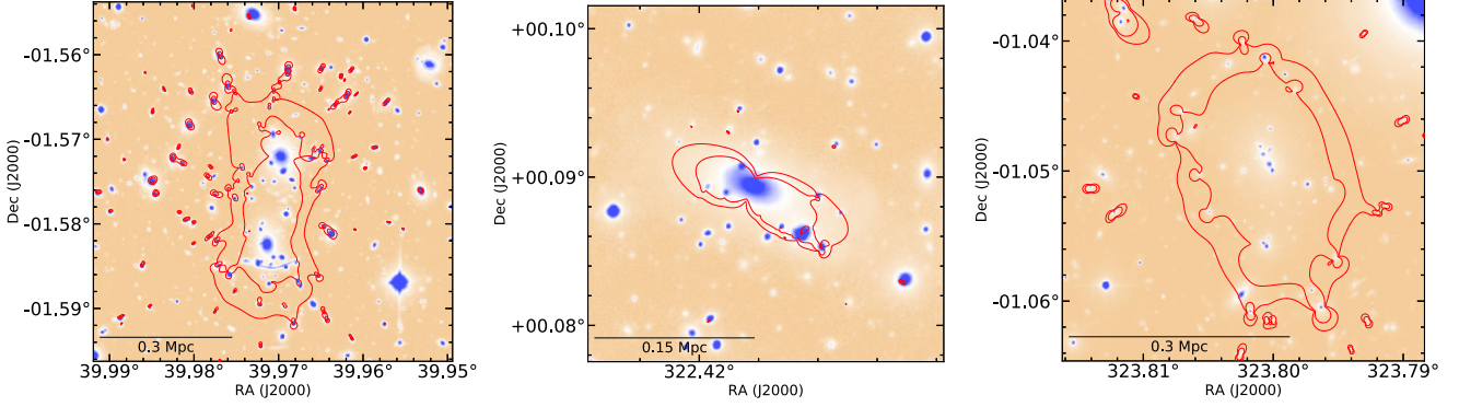
Figure 2. Central cut-outs of the Gemini GMOS z' -band images of Abell 370 (left panel), RX J2129.6+0005 (middle panel), and MACS 2135.2–0102 (right panel). North is up and east is to the left. Critical curves are plotted as red lines, and mark the location of infinite magnification for source redshifts of z = 1 and z = 2 .
