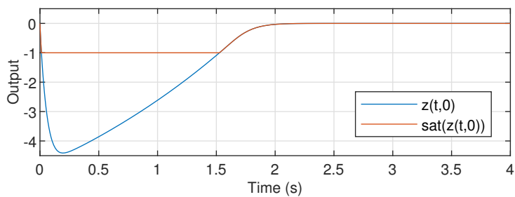
FIG. 1. Time evolution of the closed-loop system
