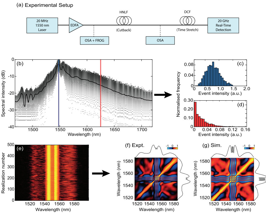
Figure 3. Typical DFT results for the real-time characterization and statistical analysis of spectral fluctuations in nonlinear fiber optics. The DFT technique, via the setup shown in (a), can be used to study a variety of dynamics highly sensitive to noise fluctuations, from a fully developed broadband incoherent supercontinuum (top) to, e.g., the onset phase of nonlinear propagation where spontaneous modulation instability takes place (bottom): (b) DFT experimental characterization of an extended incoherent supercontinuum, exhibiting important shot-to-shot spectral fluctuations. (c,d) The spectral intensity histograms reconstructed at different wavelengths exhibit very different distributions and illustrate how particular spectral regions are prone to the appearance of statistically rare ‘extreme’ events. (e) Spectral fluctuations of MI sidebands sequentially recorded by DFT. The statistical analysis of these fluctuations can be leveraged to reconstruct a map of spectral correlation (f) that can be directly compared to the same Pearson correlation maps obtained from stochastic Monte-Carlo simulations (g). Adapted from Ref. [24].
