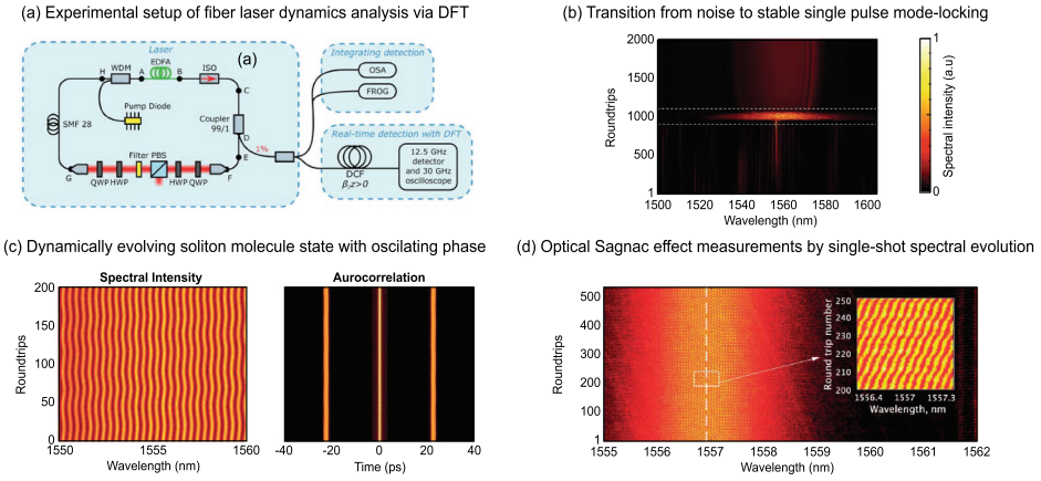
Figure 7. Examples of fiber laser evolution dynamics characterized via DFT analysis over hundreds of cavity roundtrips. (a) Experimental setup for the study of a fiber laser exhibiting soliton-similariton dynamics via DFT. (b) Single pulse mode-locking obtained after a transition from a noisy operation and an explosion regime (white dashed box), with an abrupt spectral broadening clearly captured by DFT measurements. (c) DFT measurements can be used to study the dynamical evolution of a soliton molecular state. The spectra evolution can be used to retrieve autocorrelations of the field, stemming from a ‘molecule state’ with a periodically oscillating phase. Panels (a-c) are adapted from [91]. (d) Experimental observation of the Sagnac effect in a bidirectional fiber laser, illustrated by a change in the tilted modulation pattern within the DFT spectra. Adapted from [103].
