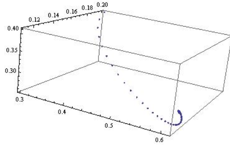
Figure 1: \alpha = 0.2, b = 0.6, \beta_1 = 0.5, \beta_2 = 0, k_1 = 1, k_2 = 0.3, x^0 = 0.1, u^0 = 0.01, y^0 = 0.2, \lim_{n \rightarrow \infty} V^{(n)}(\lambda^0) = \lambda_1. Figure 2: \alpha = 0.2, b = 0.1, \beta_1 = 0.5, \beta_2 = 0, k_1 = 1, k_2 = 0.3, x^0 = 0.3, u^0 = 0.2, y^0 = 0.4, \lim_{n \rightarrow \infty} V^{(n)}(\lambda^0) = \lambda_{10}.
