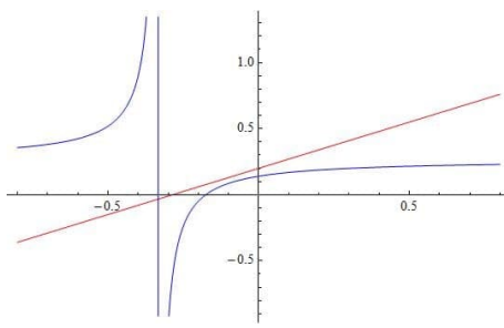
Figure 4: \beta_1 k_1 < b + \alpha, b(b + \alpha) > \alpha \beta_2 k_2
