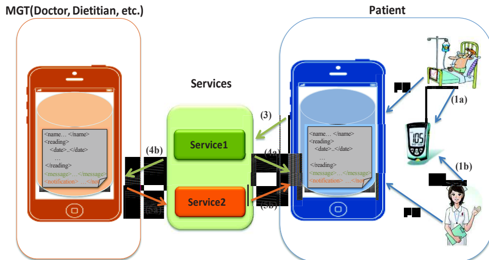
Fig. 2. ADMAN Architecture
