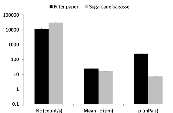
Fig. 4. Initial count number ( N_c ), mean chord length ( l_c ), and suspension viscosity ( \mu ) for FP at 1.5% w/v and SCB at 3% w/v. Error bar represents the average of the absolute deviations from their mean.
