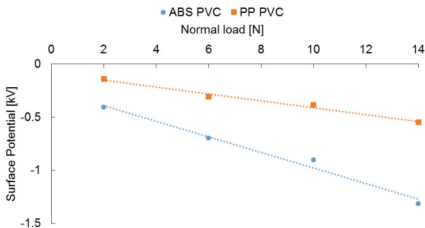
Figure 4. The average surface potential of contact area on sample (B) vs. the normal load between samples.
