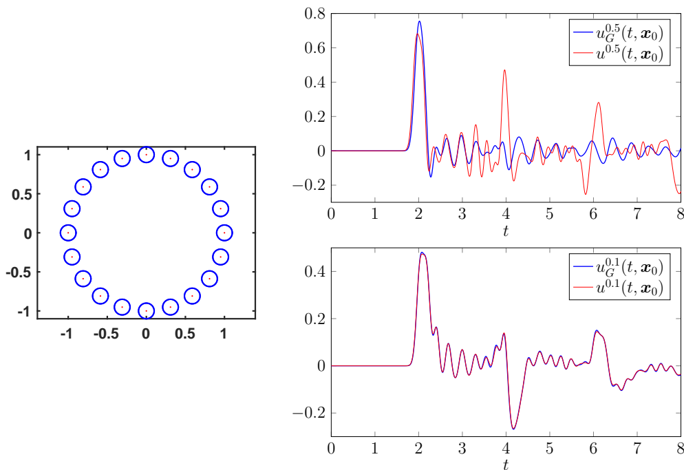
FIG. 6. Left: the geometric configuration for the numerical experiment of Section 6 for \varepsilon = 1 . Right: the dependence of the solutions u^\varepsilon(t, \mathbf{x}_0) in \mathbf{x}_0 = 0 on time t obtained with the help of the Galerkin Foldy-Lax method and the high-order BEM for \varepsilon R = 0.05 (top) and \varepsilon R = 0.01 (bottom).
