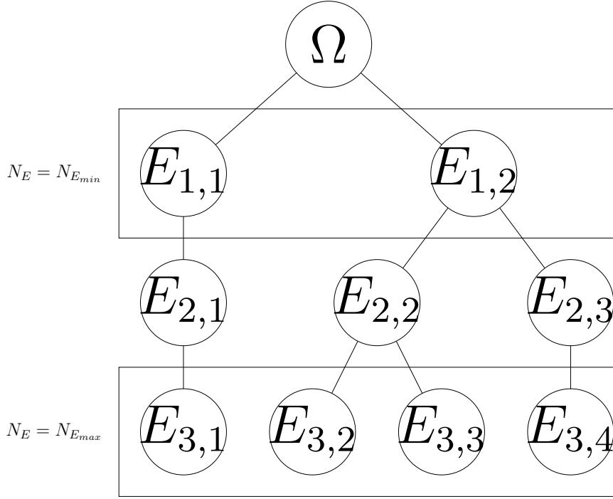
FIGURE 3 – Tree-like diagram giving an example of agglomerative clustering. Clusters are represented by circles and steps from N_E = 1 to N_{E_{max}} = 4 are displayed ; N_{E_{min}} = 2 in this example.
