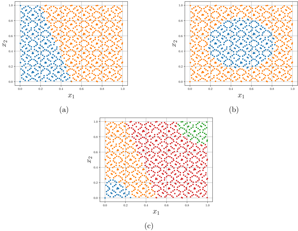
FIGURE 5 – Visualisation of 1000 labelled training observations represented in the 2D parameter space \mathcal{X} partitioned for the 3 test functions. Different colors stands for different elements obtained with the clustering. (a) Visualisation of \tilde{f}^{hyperplane} . (a) Visualisation of \tilde{f}^{hypersphere} . (a) Visualisation of \tilde{f}^{multiple} .
