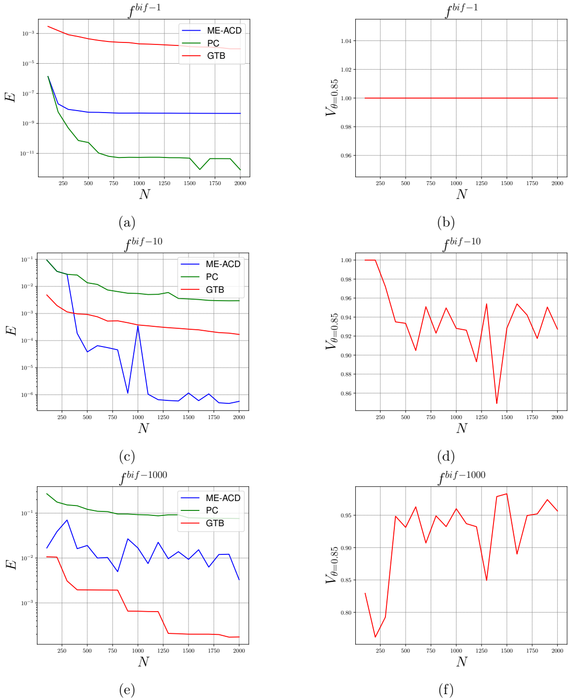
FIGURE 11 – On the left, convergence plots of the MSE between the values of the models and the true value of the 3 discontinuous functions on the test set. (a) \tilde{f}^{bif-1} . (c) \tilde{f}^{bif-10} . (e) \tilde{f}^{bif-1000} . On the right, convergence plots of the kept fraction of observations by the caution procedure of the ME-ACD on the test set. (b) \tilde{f}^{bif-1} . (d) \tilde{f}^{bif-10} . (f) \tilde{f}^{bif-1000} .
