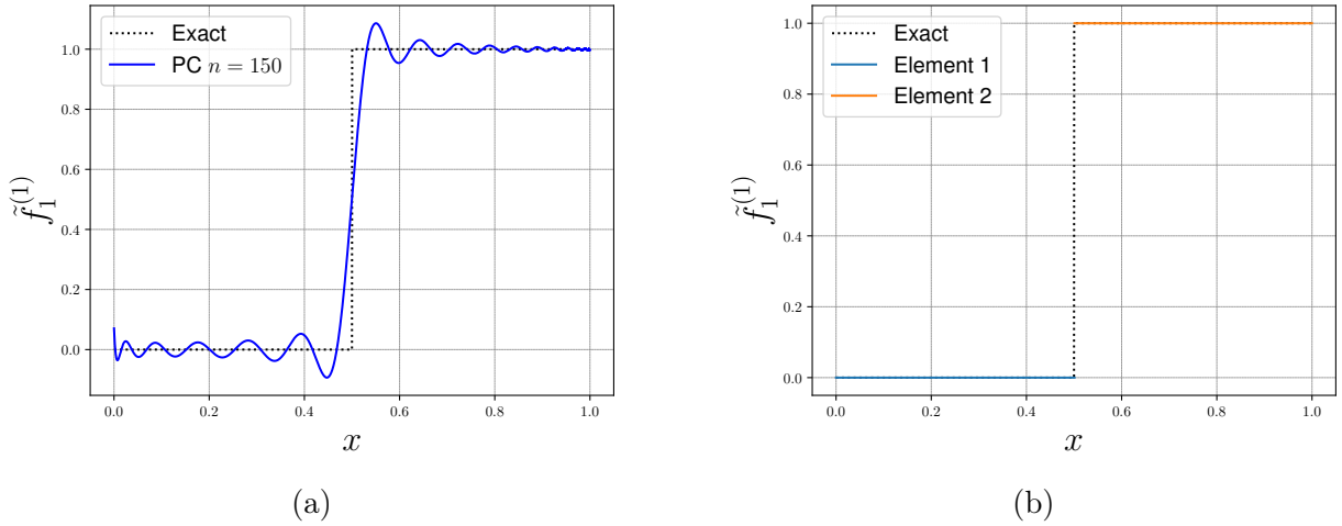
FIGURE 1 – (a) Plot of \tilde{f}_1^{(1)} (dashed lines) and of its PC surrogate model \hat{f}_1^{(1)} (plain lines) with n = 150 . (b) Plot of \tilde{f}_1^{(1)} (dashed lines) and of its piecewise polynomials model (called Multi-element model below).
