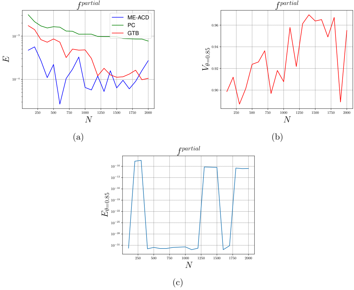
FIGURE 9 – (a) Convergence plot of the MSE for \tilde{f}^{partial} on its test set. (b) Convergence plot of the accuracy of the ME-ACD classifier and fraction of kept observations by the caution procedure of ME-ACD for \tilde{f}^{partial} on its test set. (c) Convergence plot of the MSE between the values of the models and the true value on the N_{\theta=0.85} tests observations kept by the caution procedure at each N for \tilde{f}^{partial} .
