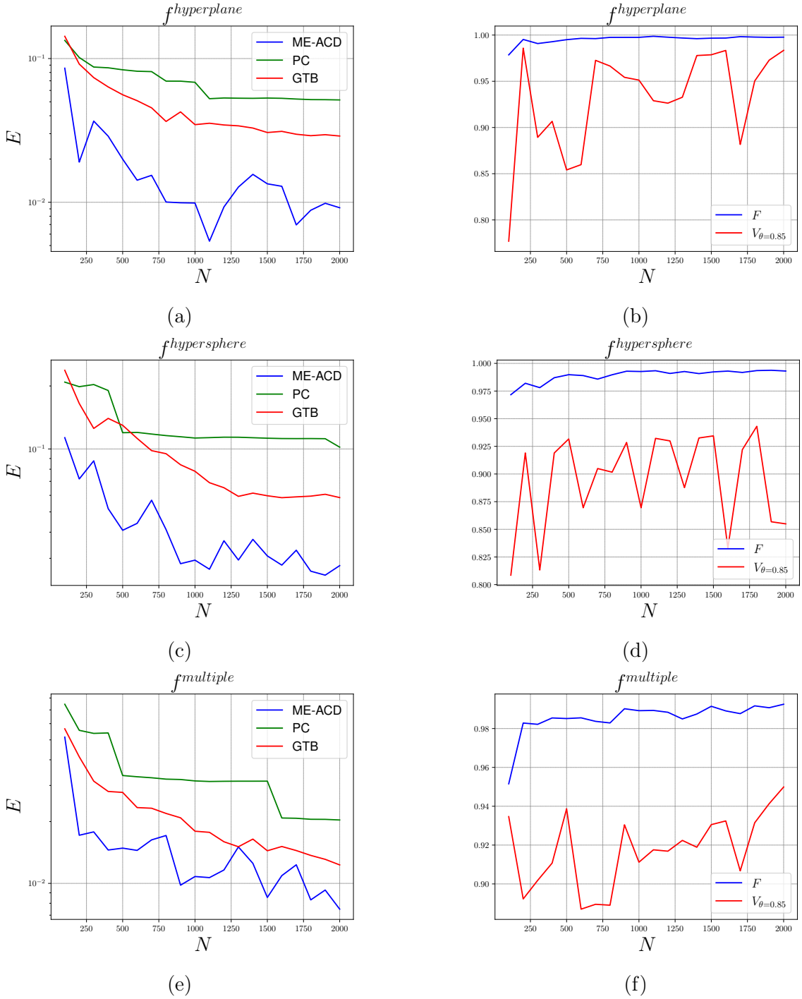
FIGURE 6 – On the left, convergence plots of the MSE between the values of the models and the true value of the 3 discontinuous functions on the test set. (a) \tilde{f}^{\text{hyperplane}} . (c) \tilde{f}^{\text{hypersphere}} . (e) \tilde{f}^{\text{multiple}} . On the right, convergence plots of the accuracy of the classifier of ME-ACD and of the kept fraction of observations by the caution procedure of the ME-ACD, on the test set. (b) \tilde{f}^{\text{hyperplane}} . (d) \tilde{f}^{\text{hypersphere}} . (f) \tilde{f}^{\text{multiple}} .
