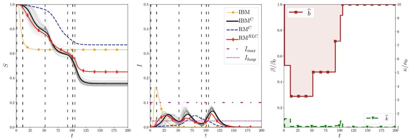
FIGURE 11 (Large population size and small dispersion) n = 0.8, \beta_0 = 0.3, \kappa_0 = 0.2, 44 iterations with (\omega_\beta, \omega_\kappa, \omega_{hosp}) = (0.5, 0.1, 0.4) . Populations with large contact heterogeneity are prone to epidemic rebounds, requiring more iterations of the proposed algorithm to meet the stopping criteria
