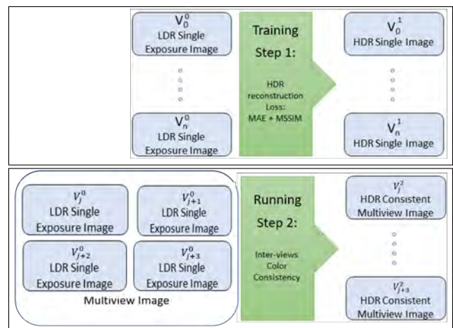
Figure 2: Our two-stage pipeline for consistent multi-view HDR reconstructions. First step: training HDR reconstruction for a single view. Second step: ensuring color consistency between views by predicting through a map containing all views. Here, V_j^i implies the j_{th} view of the results of the i_{th} step.
