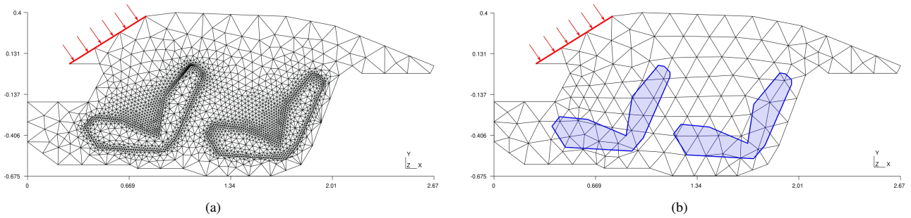
FIGURE 15 Boundary condition and meshes for the car cavity problem: (a) standard FEM model; (b) proposed approach.
