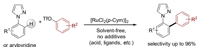
Scheme 1 Synthetic selective access to o -monoarylated azoles or pyridines under solvent- and additives-free conditions.
